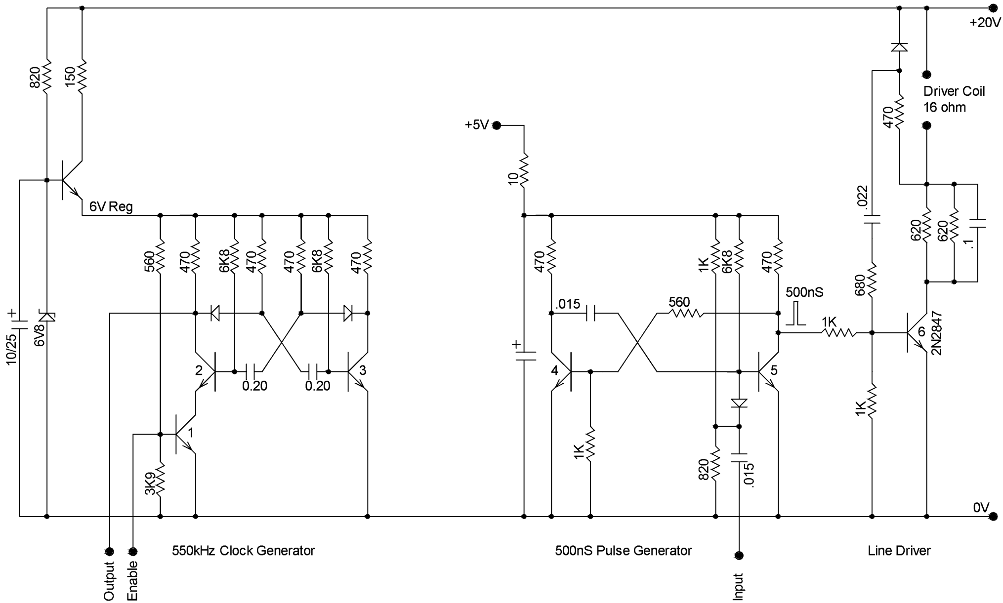
Logos 240 - Clock Generator and Delay Line Driver
